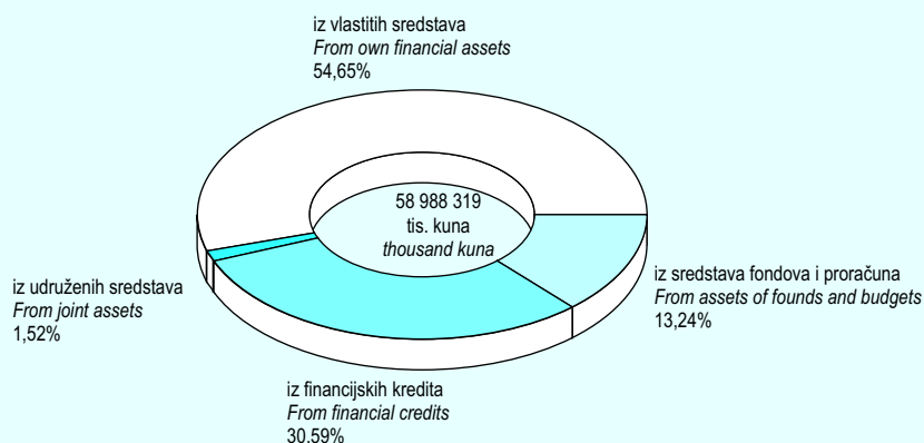
G 12-1. ISPLATE ZA INVESTICIJE U DUGOTRAJNU IMOVINU PREMA OSNOVNIM OBLICIMA FINANCIRANJA U 2005. PAYMENTS FOR GROSS FIXED CAPITAL FORMATION, BY MAIN FORMS OF INVESTMENT, 2005
